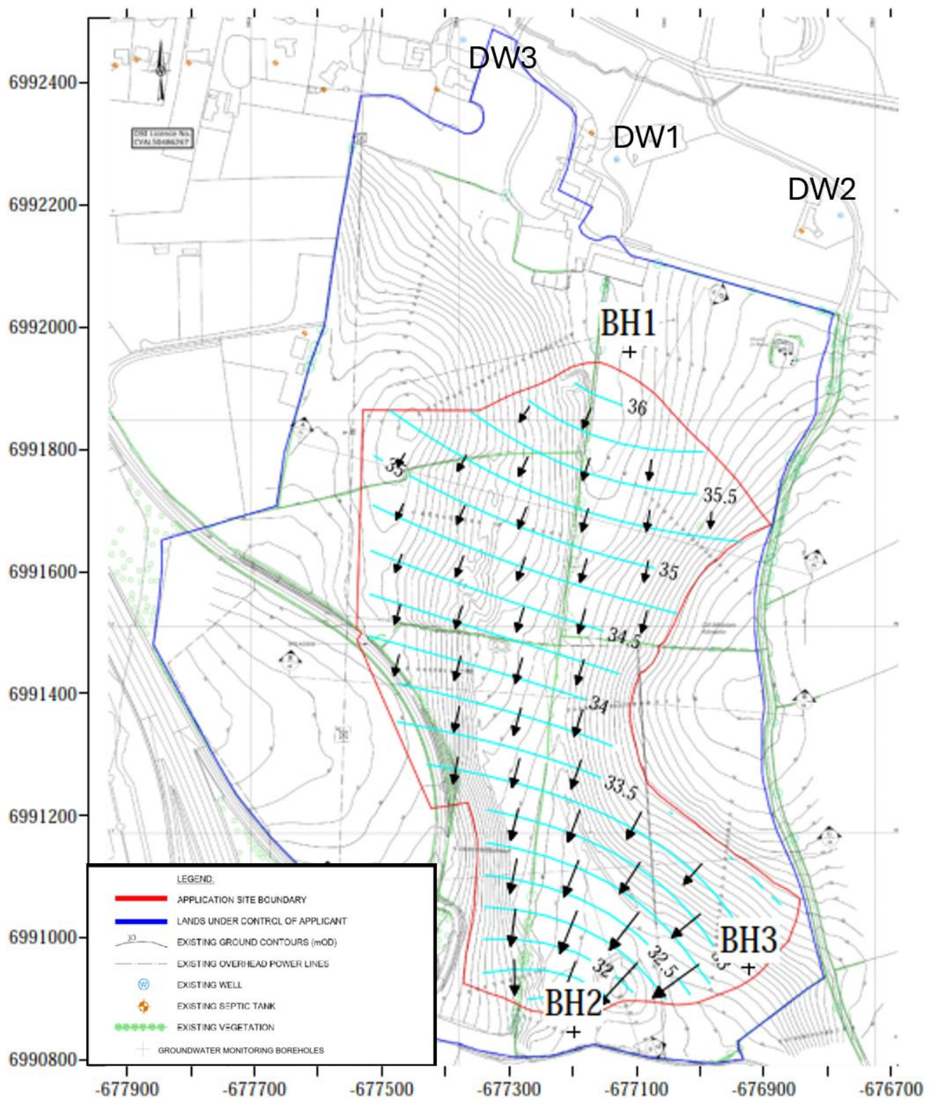
Figure 8-4 – Groundwater contours and flow direction (October 2022)
